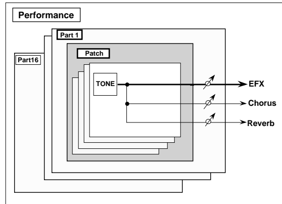
Fig.1 – When Output Assign is set to "EFX" in the Performance mode (the output settings for Tone are ignored)
